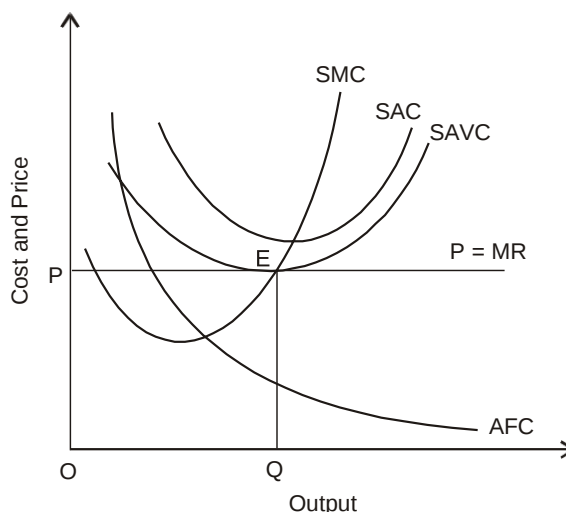
Fig. 4.4 Shut-down Point
