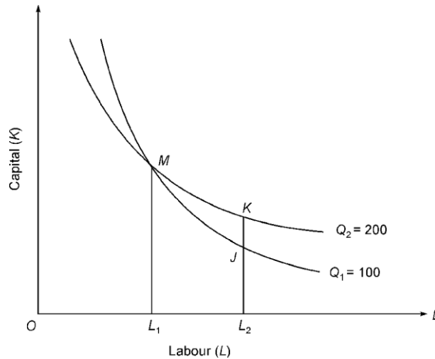
Fig. 2.4 Intersecting Isoquants
