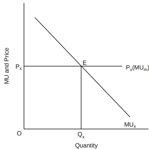
Fig. 1.2 Consumer's Equilibrium
