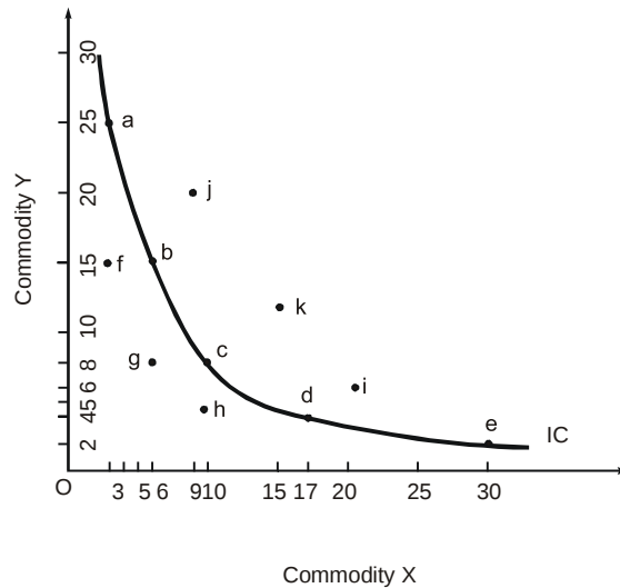
Fig. 1.8 Indifference Curve
