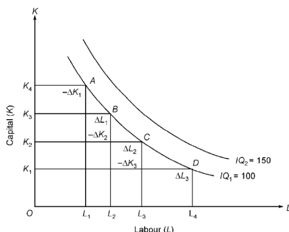
Fig. 2.3 Isoquant Curves
